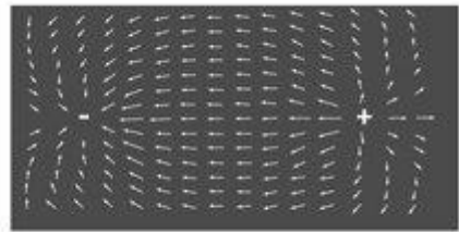
Electric field
