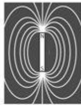
Magnetic field
