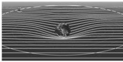
Gravitational field
